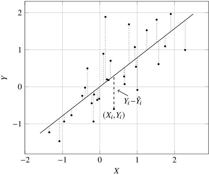
Figure 8.3 Ordinary least squares in the simple regression case. We want to minimise the squared vertical distance between each point (X_i, Y_i) and the regression line.
